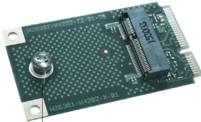
Spacer (Nut) and M3 Screw for installing the 30 mm M.2 Module (cross-head screw M3 x 3.5; bolt head \varnothing = 4.5 mm)
